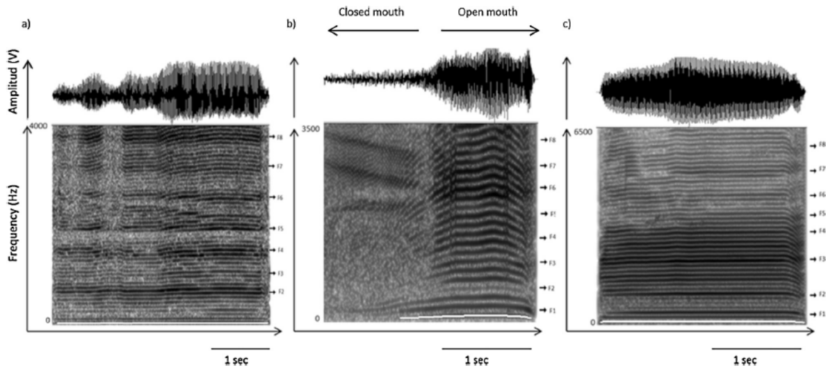
Fig. 1. Examples of oscillograms (above) and spectrograms (below) of cattle vocalisations. The white line at the bottom of each spectrogram indicates the fundamental frequency (F0). Frequency values of the formants are indicated by arrows on the right of the spectrogram. (a) Low frequency cow call produced with closed mouth (LFC). (b) High frequency cow call (HFC). The first part of the HFC was produced with the mouth partially closed, and then the second part with the mouth fully open (the arrows at the top indicate where the change occurs). For HFCs, we considered just the part with open mouth and the acoustic parameters described in this figure correspond exclusively to the acoustic analysis carried out on this part of the call. (c) Calf call (produced with opened mouth).
