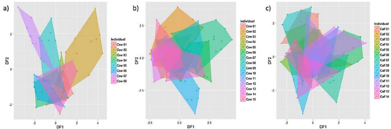
Fig. 3. (a) First two discriminant function scores for cow LFCs; n = 8 cows, with 7–10 calls per individual. Points represent individual calls, while polygons delineate areas of parameter space occupied by calls of different individuals. Cross-validated DFA classified 53.6% of calls correctly. (b) First two discriminant function scores for cow HFCs; n = 15 cows, with 7–10 calls per individual. Cross-validated DFA classified 30.9% of calls correctly. (c) First two discriminant function scores for calf calls; n = 14 calves, with 9–10 calls per individual. Cross-validated DFA classified 23.7% of calls correctly.
