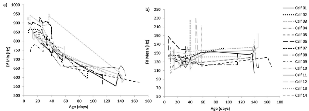
Fig. 2. (a) Effect of calf age on DfMin. Each line represents data from a different individual. ANCOVA with PC1 (which was strongly correlated with various formant characteristics, including DfMin) as the response variable showed that the effect of age and the interaction between age and individual were significant. (b) Effect of calf age on F0Mean. Each line represents data from a different individual. ANCOVA with PC2 (which was strongly correlated with F0) as the response variable showed that there was no significant effect of age.
