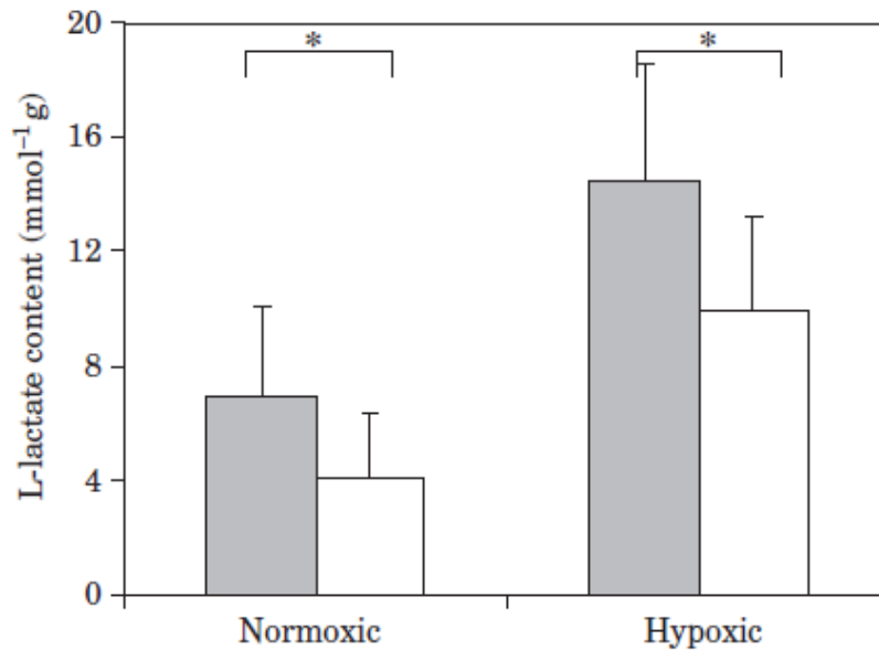
FIG. 3. Mean \pm S.D. whole body L-lactate concentrations for three-spined sticklebacks from river (■) and pond (□) populations held under normoxia and hypoxia ( n = 16 fish in each group). River fish had higher whole body L-lactate concentrations than pond fish for both treatments (*, P < 0.001 ).
